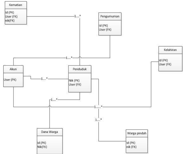
Figure 4.5 Logical Database
